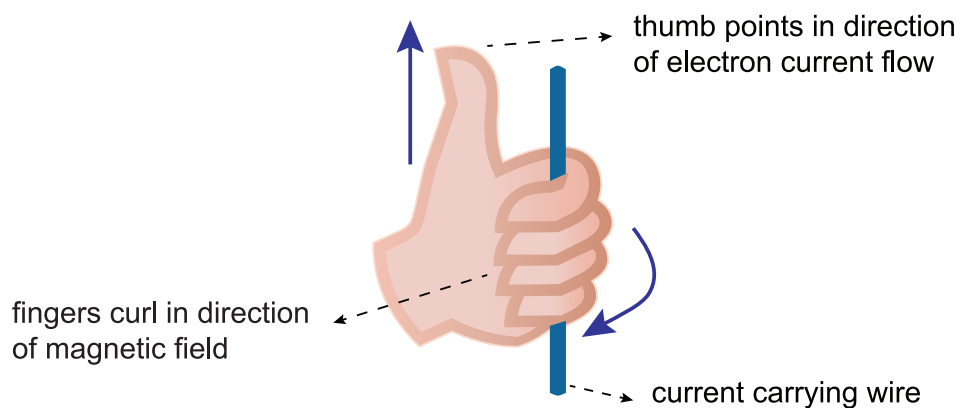
Figure 4.6: The left-hand grip rule for electron current
