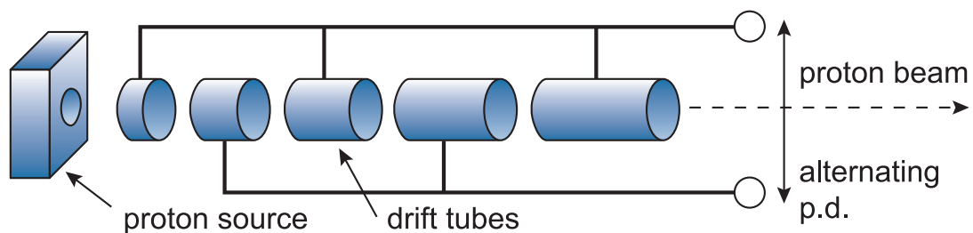
Figure 3.4: A linear accelerator
