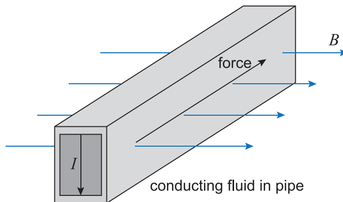
Figure 4.14: The electromagnetic pump
