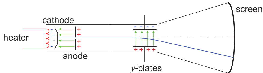
Figure 3.3: The cathode ray tube
