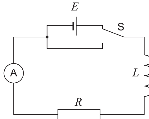
Figure 6.10: d.c. circuit with resistor and inductor in series
