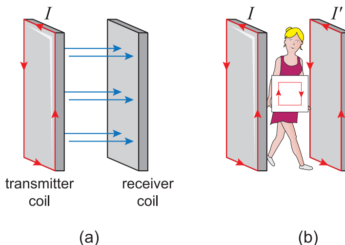
Figure 6.7: Schematic of an airport metal detector
