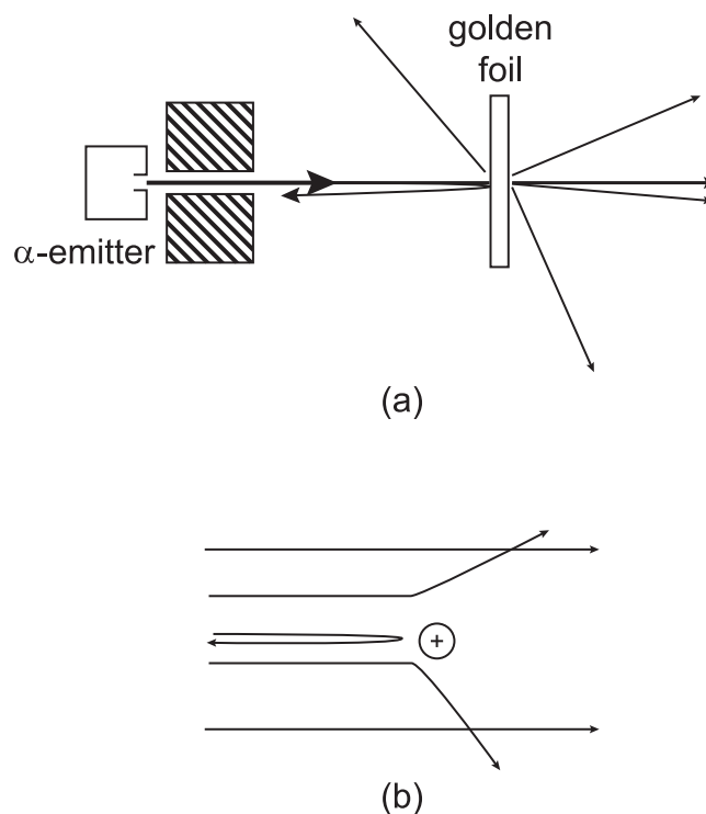
Figure 3.5: Rutherford scattering
