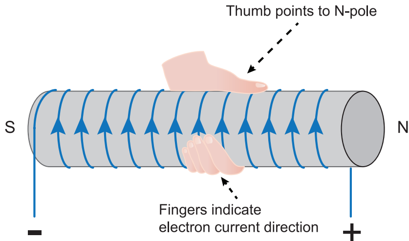
Figure 4.9: The magnetic field pattern caused by current in a long solenoid
