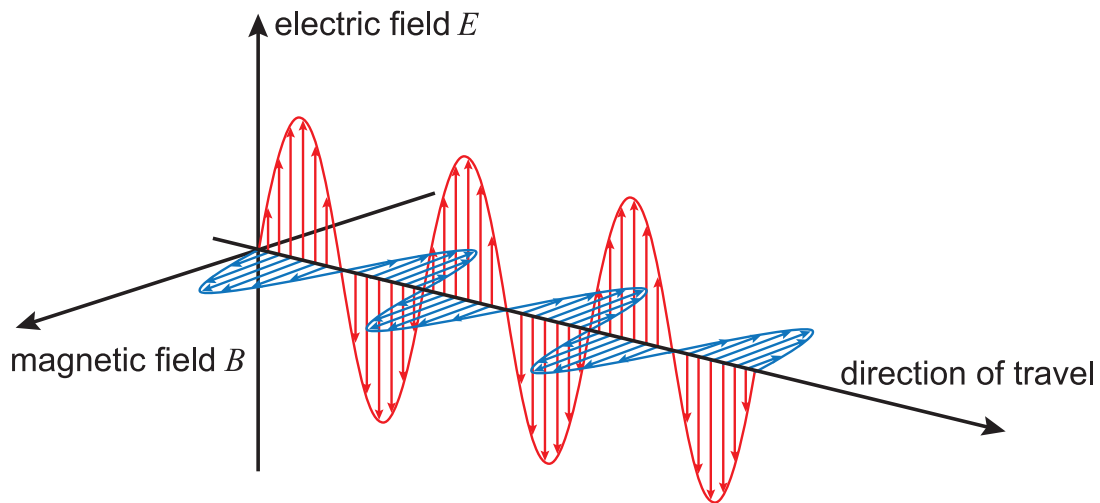
Figure 7.1: Electromagnetic wave
