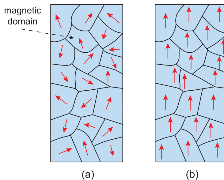
Figure 4.1: Magnetic domains
