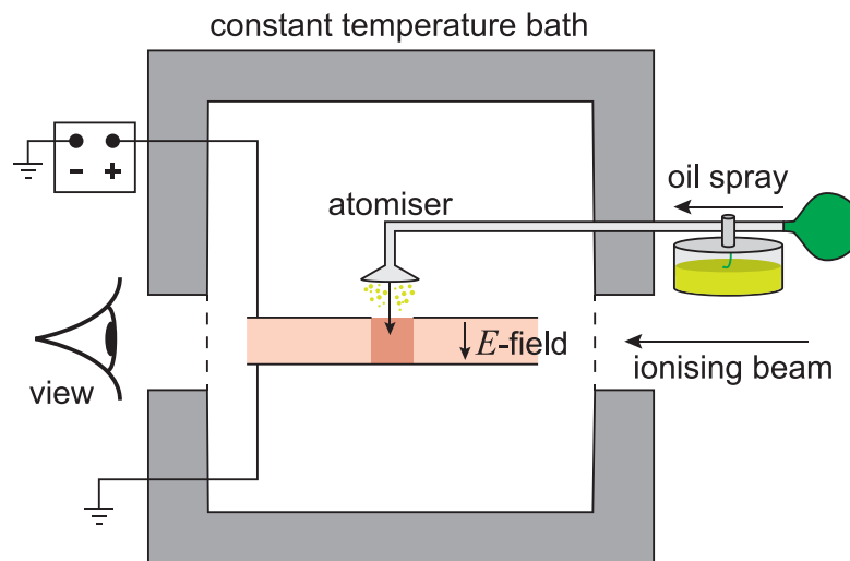
Figure 4.15: Experimental arrangement of Millikan's oil drop experiment
