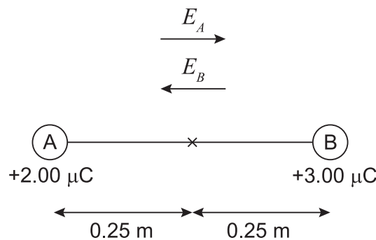
Figure 1.4: Electric fields due to two positive charges
