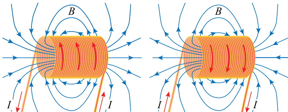
Figure 6.1: Solenoids - the direction of the current (electron flow) tells us the direction of the magnetic field
