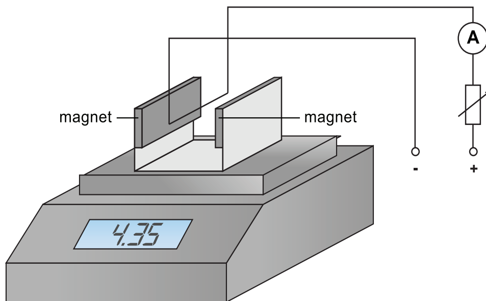
Figure 4.12: Measuring the force on a current-carrying conductor
